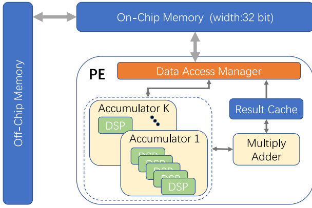
Fig. 4. The design of matrix-vector multiplication accelerator on FPGA for verifying the performance improvement brought by DP-Nets.
