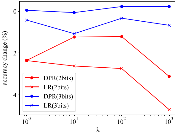
Fig. 5. The results of compressing TT-Conv with DPR. The accuracy change for varied \lambda with t = 100 .
