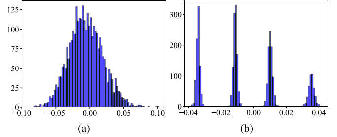
Fig. 2. The histograms of weights in the FreshNet model's first convolution layer obtained from (a) a normal training, and (b) a clustering-friendly training.
